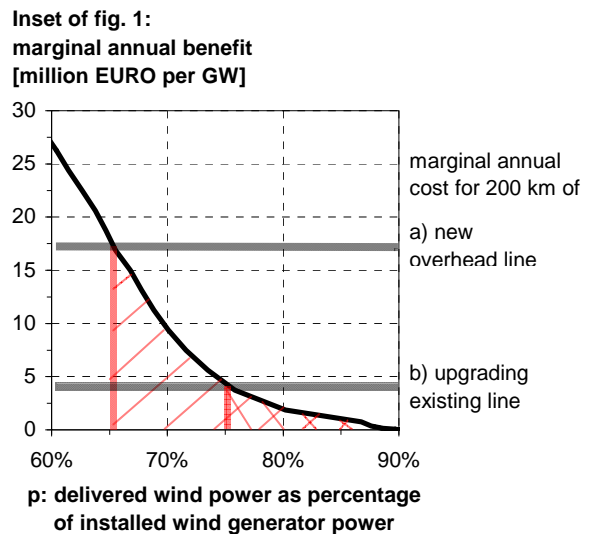
Fig. 2 : The optimum – intersection of marginal benefit and marginal cost curves
