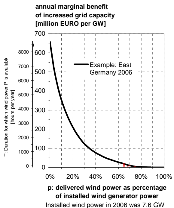
Fig. 1 : Duration-power-curve
